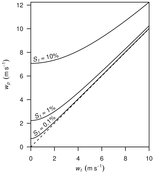
Figure 1. The velocity w_p of polluted updrafts from Equation 1 using a/rc_d = 1,000 \text{ m}^2 \text{ s}^{-2} plotted as a function of the velocity w_t of typical updrafts for three different values of the typical supersaturation S_t : 0.1%, 1%, and 10%. For visual reference, the dashed line marks w_p = w_t .
